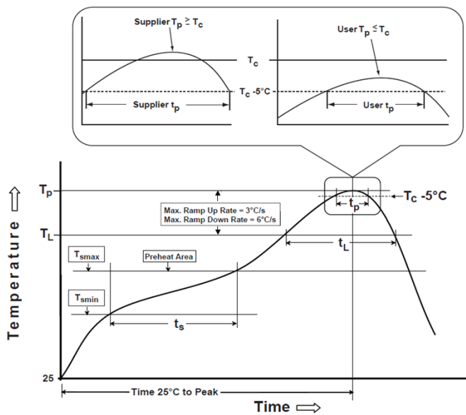
Fig.1 Soldering Reflow
